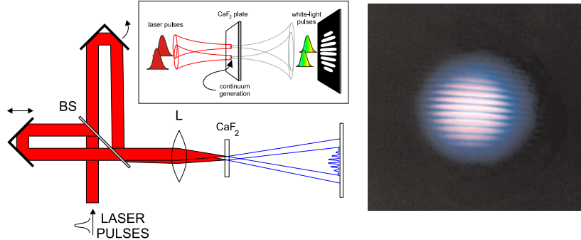
Figure 1.6. Scheme of the experiment for the observation of white-light interference fringes. The two pump pulses are generated by the same laser system and by the same Michelson interferometer described above. Two independent SC pulses are generated in the material and then propagate and overlap on a screen. A snapshot of the observed interference pattern is also shown, taken with an exposure time of about 2 seconds and with a laser repetition rate of 1 kHz. The very good visibility of the fringes indicates that the phase lock is not only preserved on a shot-to-shot basis, but that a constant phase relationship is maintained over at least thousands of shots.
