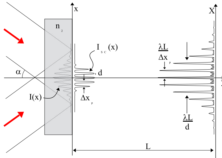
Figure 1.12. Sketch of the experimental setup illustrating the geometry of the interaction. Two laser pulses intersect at an angle \alpha and form an interference pattern on the x plane inside the material. The maxima of this interference pattern become the sources for supercontinuum radiation which propagates to a screen placed at a distance L .
