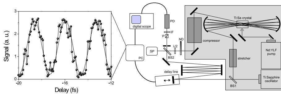
Figure 1.15. Experimental setup. The shaded area delimits the amplified laser source. ND: variable neutral density filter; P: cube polarizer; \lambda/2 : half-wave plate; IF: narrow-band interference filter; PD: fast photodiode; SP: spectrometer; BS1 and BS2: 50% beam splitters; PC: personal computer. Also shown is the interference signal (filled circles) obtained while scanning the delay between the original laser pulse and its amplified replica. The solid line is a fit to a sine function.
