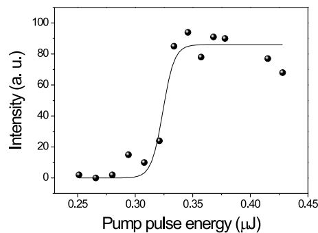
Figure 1.8. Behavior of the SC intensity variation as a function of the incoming laser pulse energy for a wavelength of about 550 nm. Filled circles are experimental data while the solid line is a fit with an hyperbolic tangent function.
