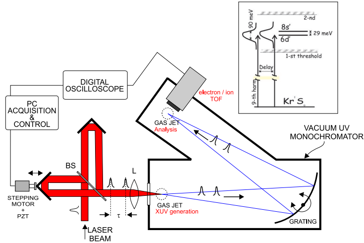
Figure 1.4. Experimental set-up and scheme of the interaction (inset), showing the involved autoionizing levels of the krypton atom: the ninth harmonic, generated by focusing the phase-locked pulse pair in the xenon jet is selected by the monochromator grating and crosses the krypton jet in the interaction chamber. The electrons ejected in the one-photon ionization process are energy-analyzed by a TOF spectrometer
