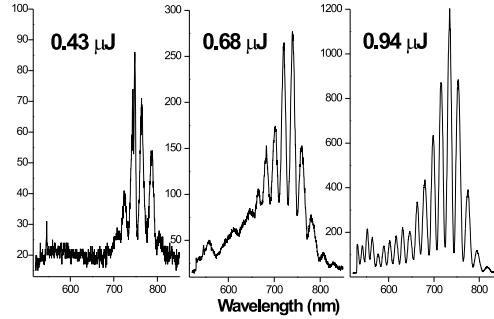
Figure 1.7. Appearance of white-light spectral interference fringes on the visible side of the laser spectrum in a 1-mm thick glass plate. In the sequence of spectra measured at different single-pulse energies, one can observe the birth of a single supercontinuum pulse and the appearance of the second, phase-locked, pulse which produces a clear sinusoidal modulation in the spectrum.
