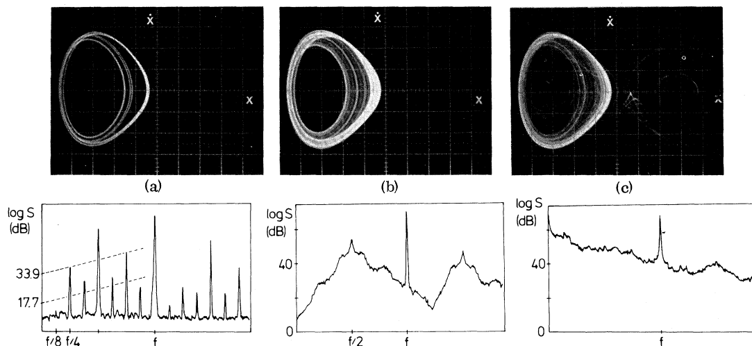
FIG. 1. Three examples of nonlinear motion for a modulation frequency f = 575.2 Hz. Row I: phase-space plots [horizontal x(t) ]. Row II: power spectra in log (vertical)-linear (horizontal) scales. (a) V = 642.76 mV, line spectrum; (b) V = 649.12 mV, one strange attractor, broad spectrum with low-frequency cutoff; (c) V = 685.56 mV, two strange attractors, low-frequency divergence.
