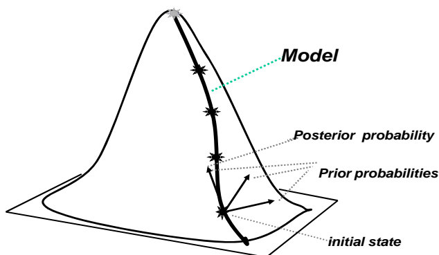
Fig.1- Apprehension as a Bayes inference. One formulates a manifold of hypotheses; each one provides a datum through the top-down conditional probability; only the hypothesis that generates the actual datum (bottom-up) is the plausible one.
