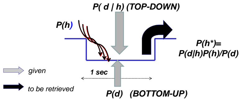
Fig.1- Apprehension as a Bayes inference. One formulates a manifold of hypotheses; each one provides a datum through the top-down conditional probability; only the hypothesis that generates the actual datum (bottom-up) is the plausible one.
