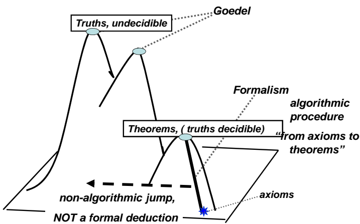
Fig.4. The semantic complexity explains the criticism of K. Goedel to Hilbert's formal deduction of theorems as the only way to extract truths from a body of axioms.
